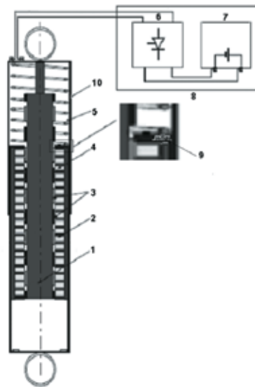
Fig. 1. Electromagnetic shock absorber; 1 - rod with permanent magnets, 2 - cylinder with set of coils, 3 - permanent magnets, 4 - coil, 5 - hollow spring with electric wires inside, 6 - controlled rectifier, 7 - battery, 8 - energy storage, 9 - wiring terminals, 10 - cover
