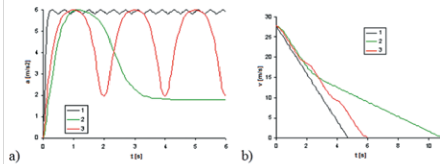
Fig. 3. Values of a) deceleration and b) velocity of automobile against time for three modes of the braking process. 1 - with using ABS system, 2 - pulse braking, 3 - braking with wheels locking
