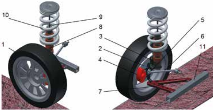
Fig. 2. McPherson's column as the dynamical set of two degrees of freedom; 1 - wheel, 2 - brake disc, 3 - steering, 4 - brake caliper, 5 - joint, 6 - drive half-axle, 7 - arm, 8 - stator of the shock absorber (cylinder of shock absorber), 9 - rod with permanent magnets, 10 - spring, 11 - car chassis
