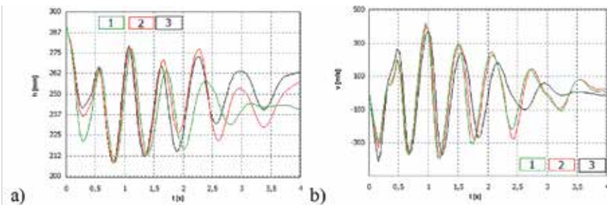
Fig. 4. Values of a) displacement and b) velocity of the shock absorber ends vs. time for three modes of the braking process. 1 - with using ABS system, 2 - pulse braking, 3 - braking with wheels locking
