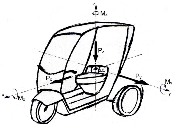
Fig. 6. The forces and moments applied to the three-wheeler as loads (s.c. = cg = centre of gravity – translator's note)
