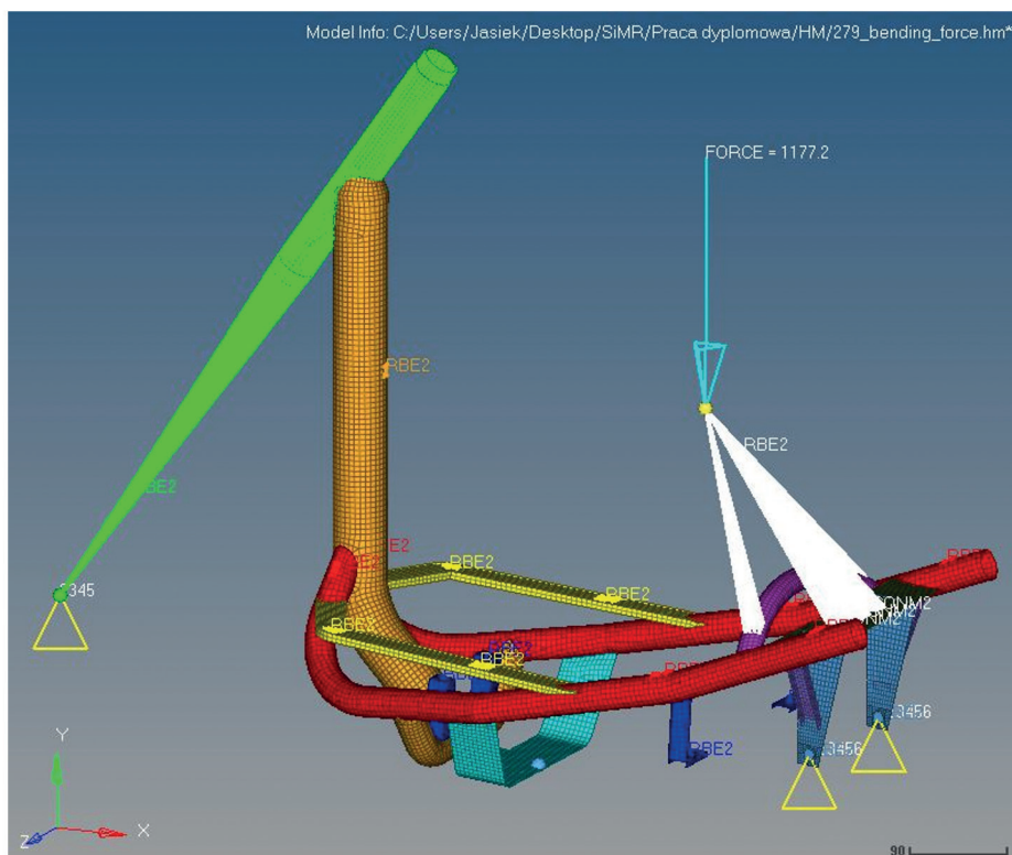
Fig. 13. Loading the vehicle frame when determining its bending stiffness [source: authors' materials]
