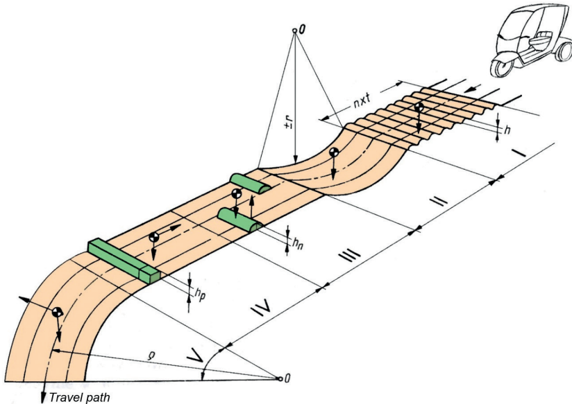
Fig. 7. Model of the road, which represents the basic events occurring on roads
