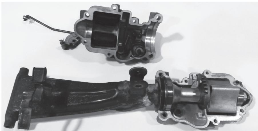
Fig. 4. Tilting swingarm used in the Honda Gyro motorcycle [source: authors' materials]
